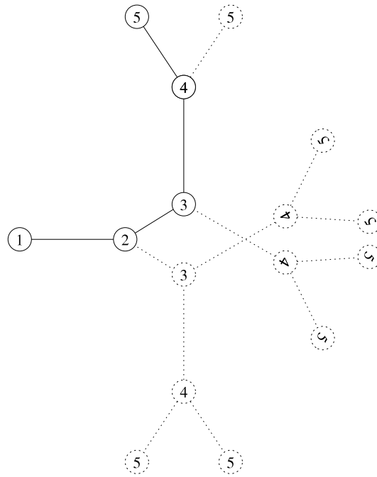
Fig. 1. All 8 possible embeddings of a 5 vertex instance. The embedding described by the bit-string 000 is depicted with solid lines.
