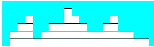
Fig. 4. Illustration of laminar intervals.
