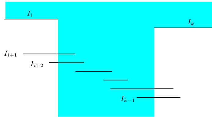
Fig. 2. The subinstance \mathcal{J}_{i,k} .
