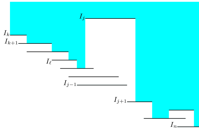
Fig. 3. Recurrence relation of C_k . If I_j is the first E-interval after I_k , then the cost divides into the cost of the intervals between k and j , plus C_j .
